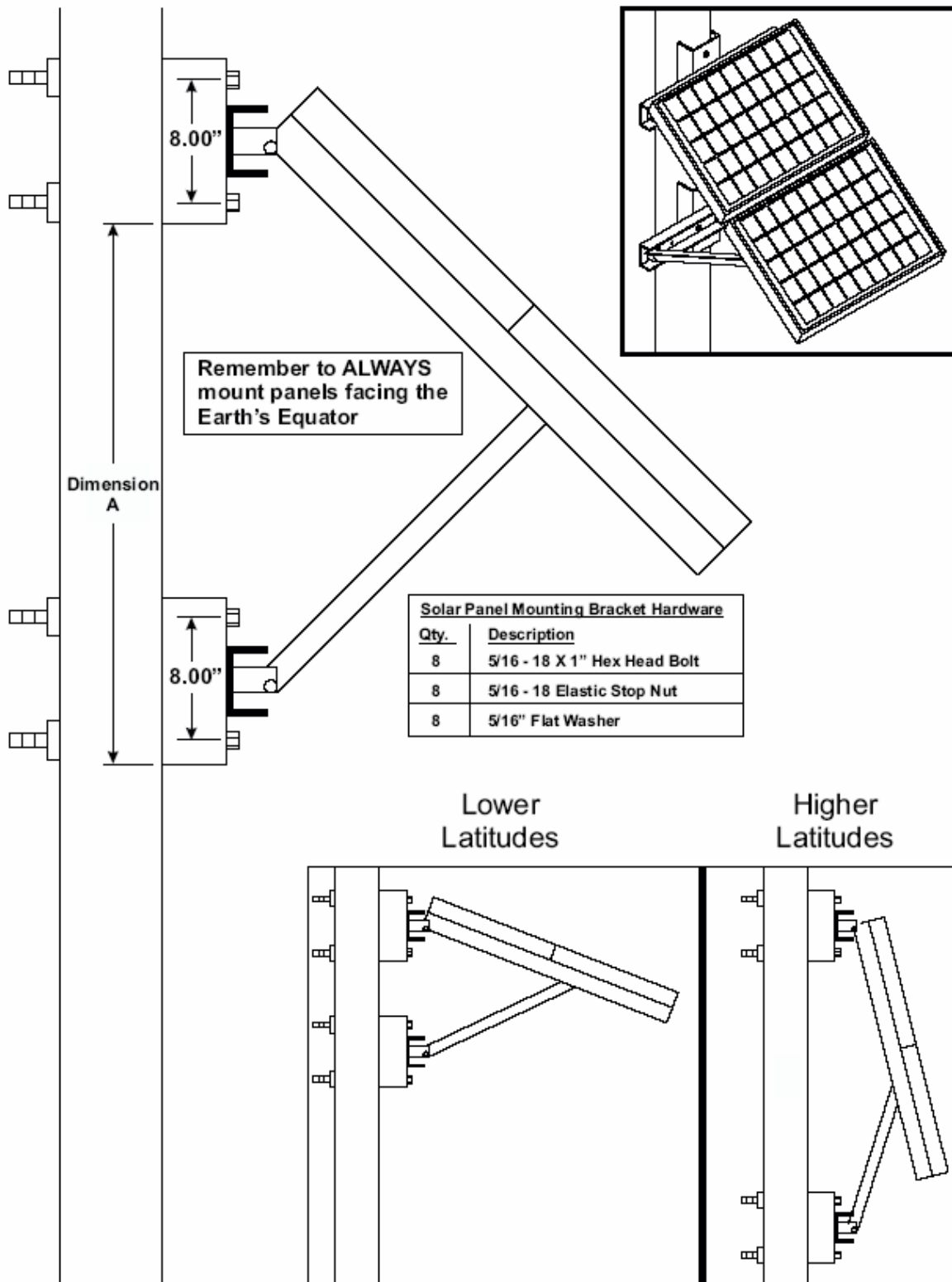
Fig. 9: Solar Panel Mounting Views
