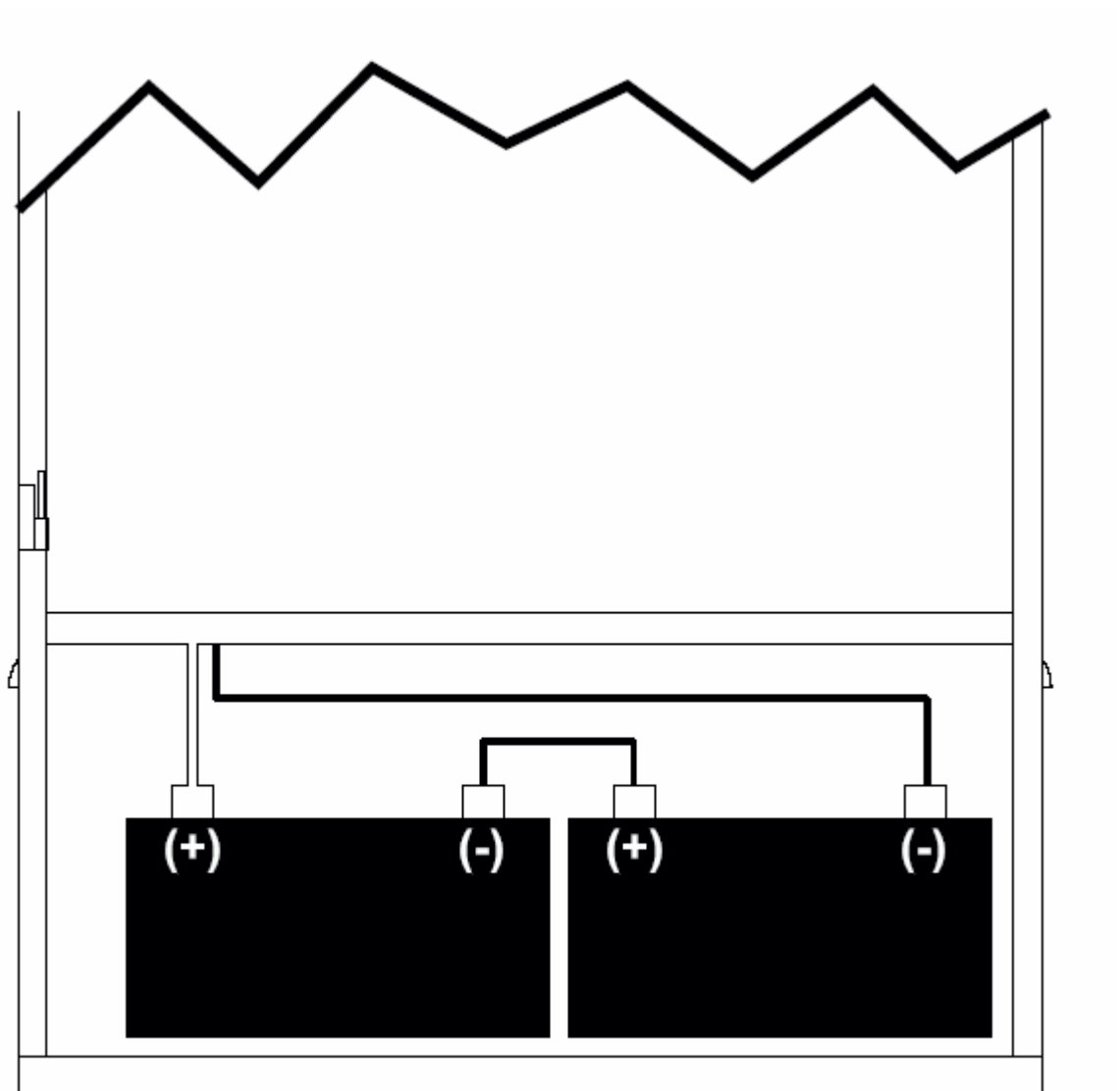
Fig. 12: Battery Connections
