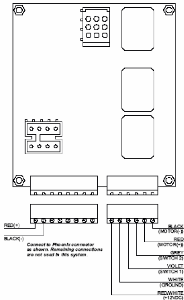
Fig. 10: Oscillator Board Connections
