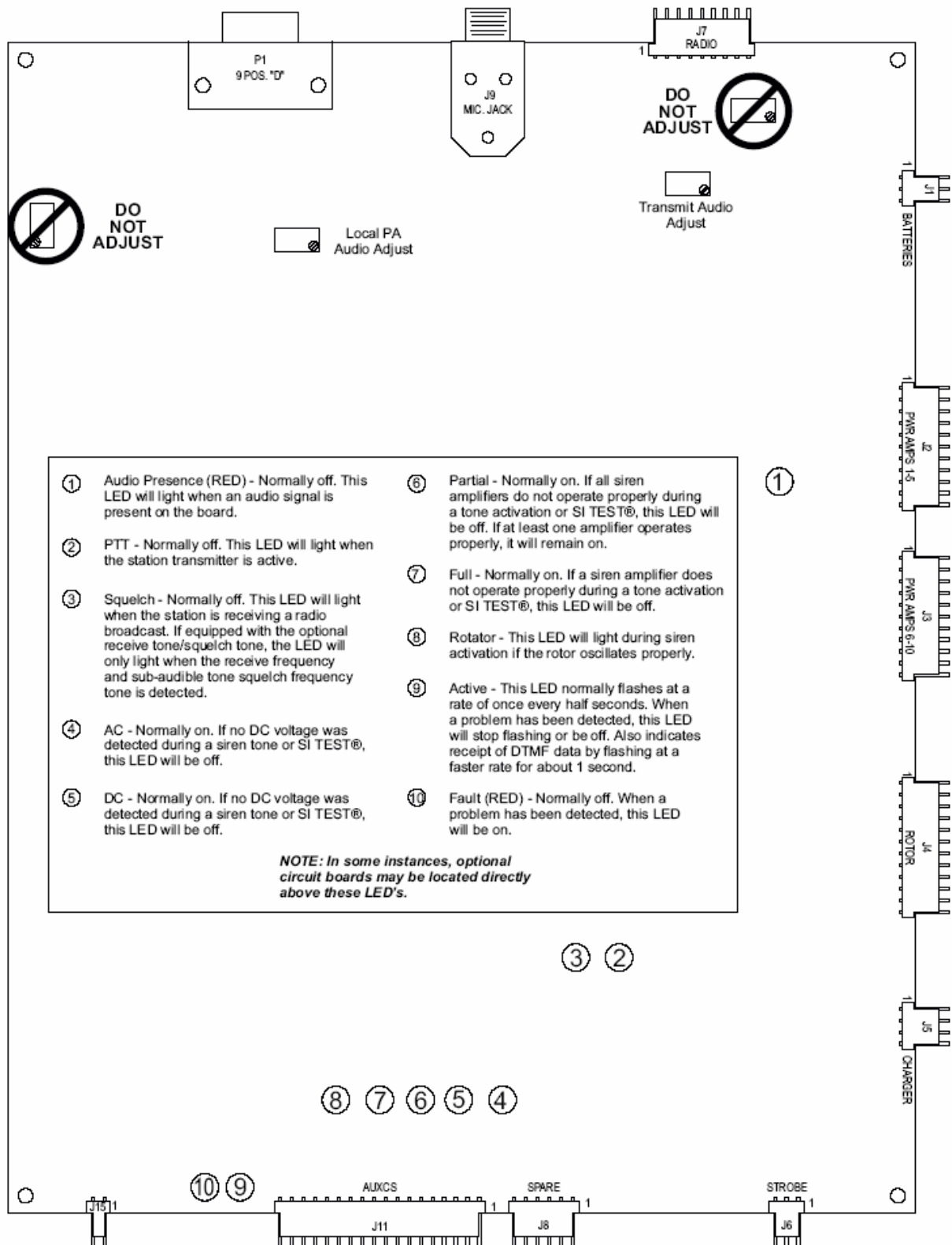
Fig. 16: System LED Diagnostic Indicators
