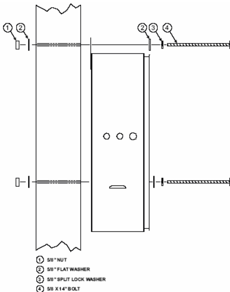
Fig. 5 Electronic Cabinet Mounting (Side View)
