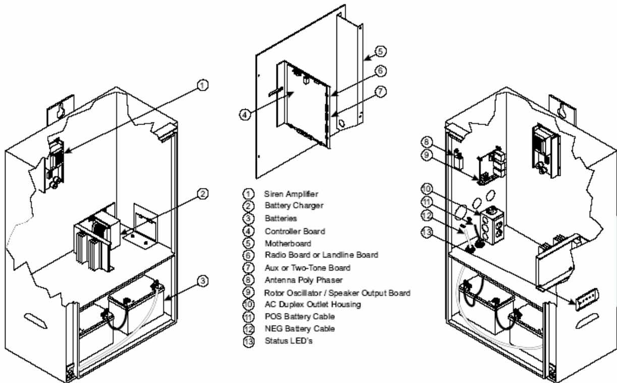
Fig. 17: Siren Cabinet Components
