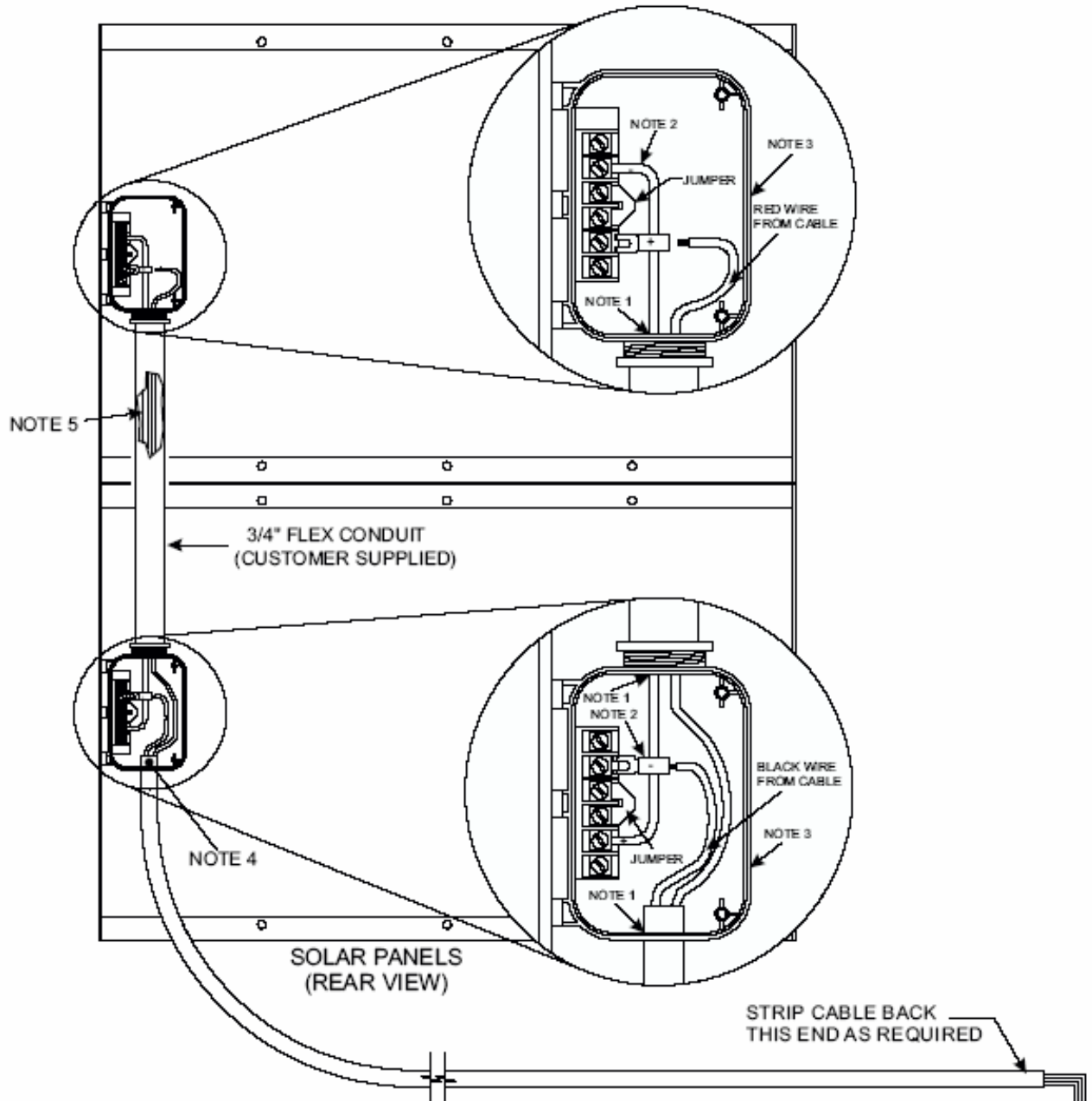
Fig. 8: Solar Panel Wiring Connections
