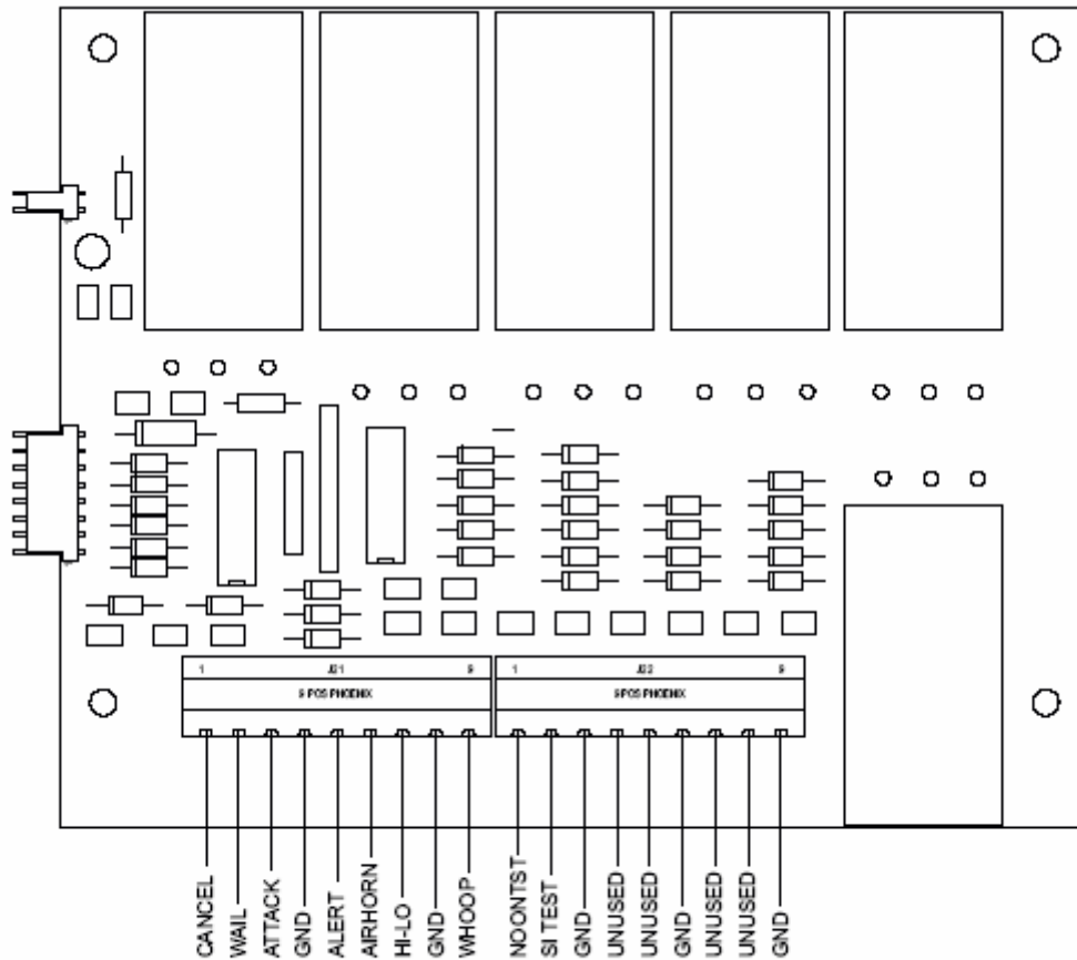
Fig. 15: Aux-In Board
